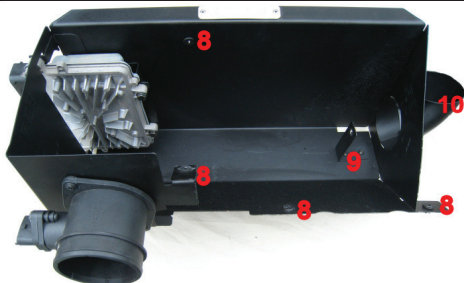
11. Assemble the 6 plastic clips to the plate (8). Assemble the air mass meter, the ECU and the curved pipe (10) to the OptiFlow heat shield. Assemble the rod (9). (as picture shows)
