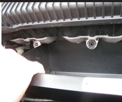
14. Tighten the heat shield, start with the two attach points to the left, leave the third for later
