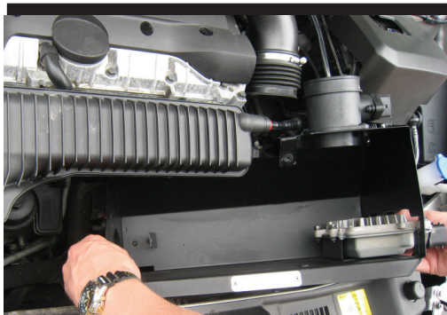
13. Assemble the OptiFlow heat shield to the car, slide it down from right to left. Fit the steering pin under the OptiFlow heat shield to the rubber bushing (See pic 11 point 6).
