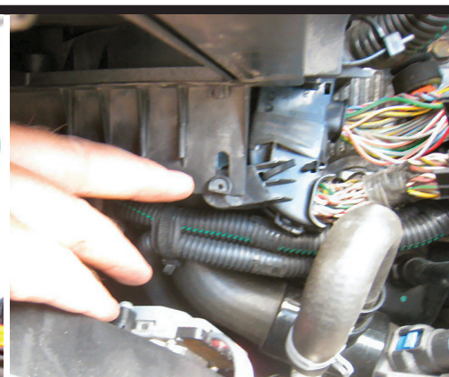
6. Remove the cable harness from the air filter box.
