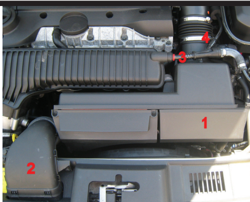
2. Remove the plastic cover (1) above the ECU by pulling. Remove the inlet tubing (2). Remove screws and turn pipe 45° clockwise. Remove the inlet pipe (3) from the inlet by pushing the red ring and at the same time pulling the pipe. Remove the hose (4) from the air mass meter.
