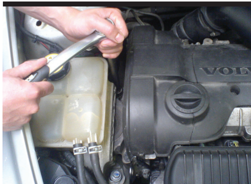
7. Remove the two bolts from the right hand side engine mounting. Remove the protective cover from under the engine. Put the car jack under the oil pan and lift up the engine slightly, max 10-15mm. Push the engine backwards.
