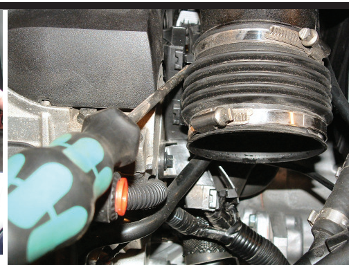
9. Cars with automatic gear box: Open the electrical harness cover.
