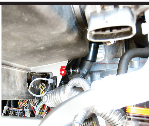
5. Remove the cable harness from the air filter box. Cut of the tie wrap holding the harness. Remove screw (5).
