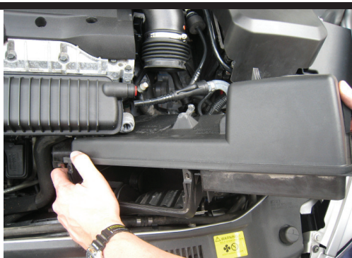
8. Pull the airfilter box straight up until lets go of the rubber bushing. Then pull the box to the left and turn it at the same time upwards to release it. Remove the ECU and the air mass meter from the air filter box.
