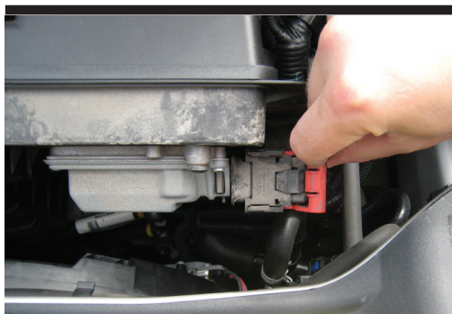
4. Remove the connectors from the ECU. Loosen both of the red clips and pull the connectors.
