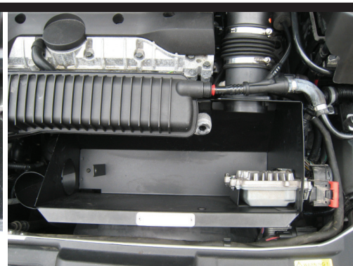
15. Assemble the harness connector and the air hose to the air mass meter. Assemble the two harness connectors to the ECU. Snap on the red locks. Assemble the vacuum pipe to the inlet.
